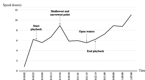
Figure 3. Horizontal average speed recorded for the rescued killer whales as they progressed throughout the shallow inlet and out in open waters, calculated as the ratio between the distance and time between two successive sightings of surfacing killer whales
